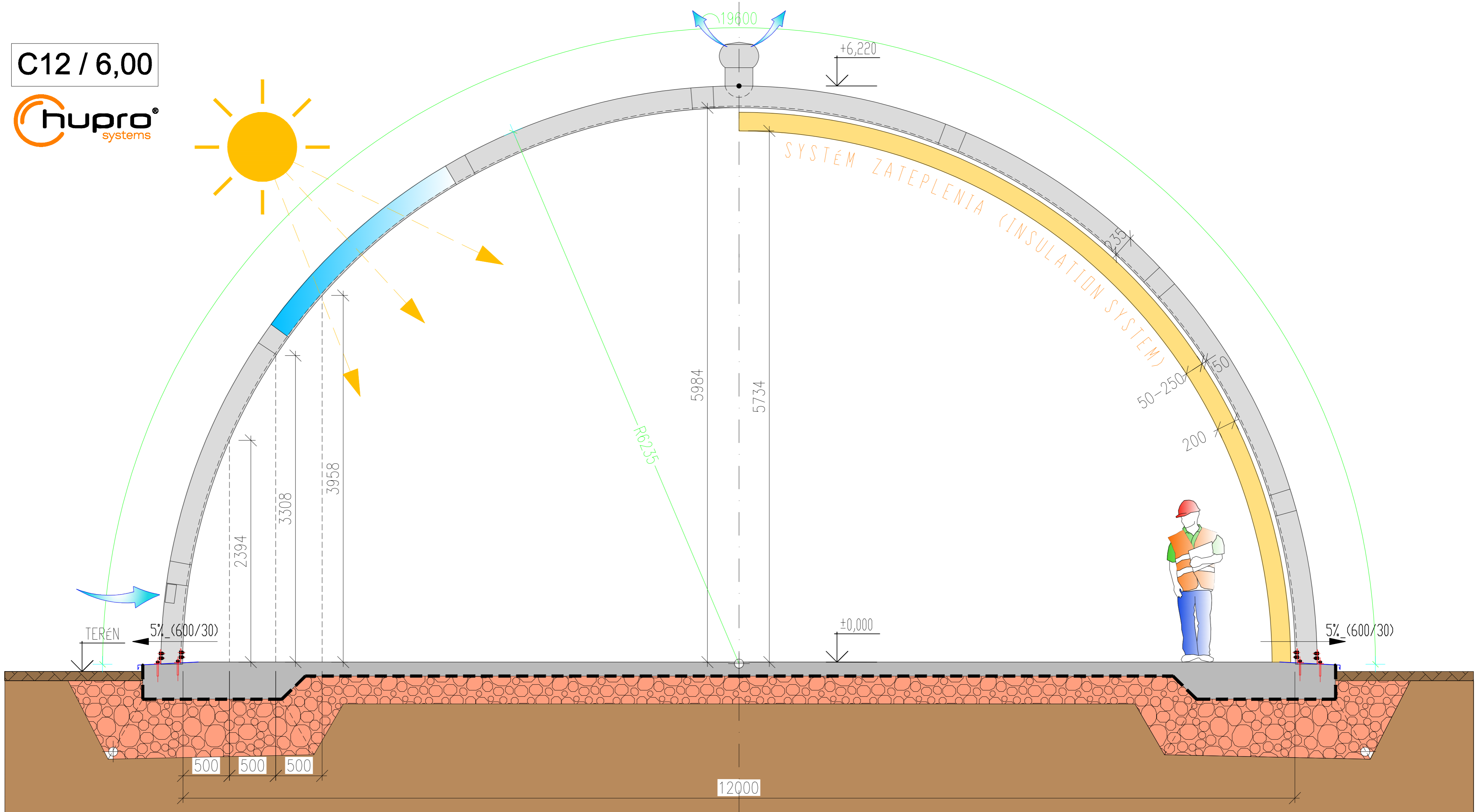
ORIENTAČNÝ TVAR ZAKLADANIA (ORIENTATION FORM OF FOUNDING)
